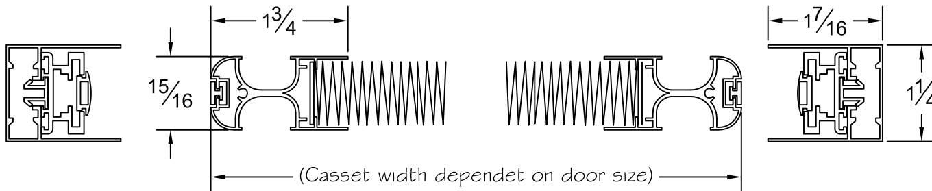
Horizontal Section View
